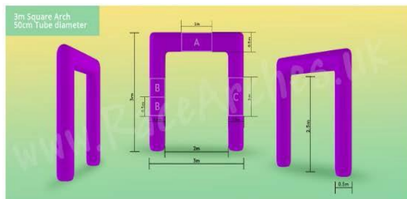
3m Square Arch
