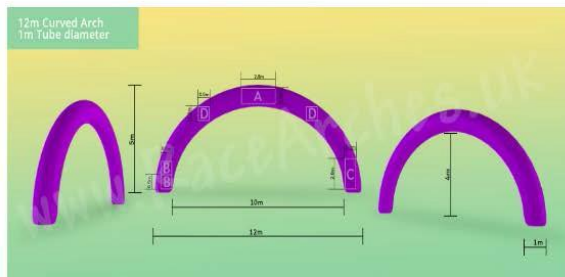
12m Curved Arch
