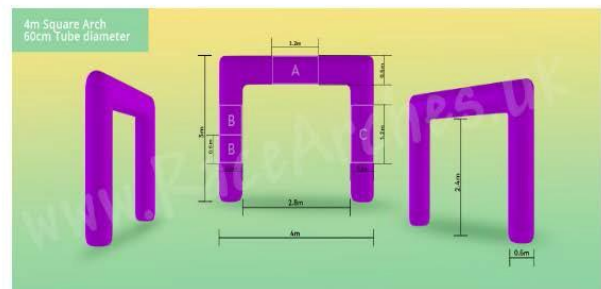
4m Square Arch
