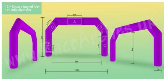
10m Square Angled Arch
