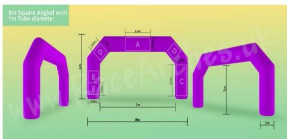
8m Square Angled Arch
