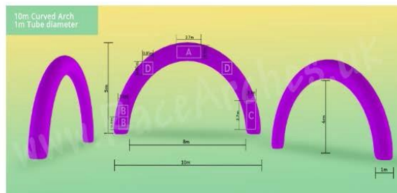
10m Curved Arch
